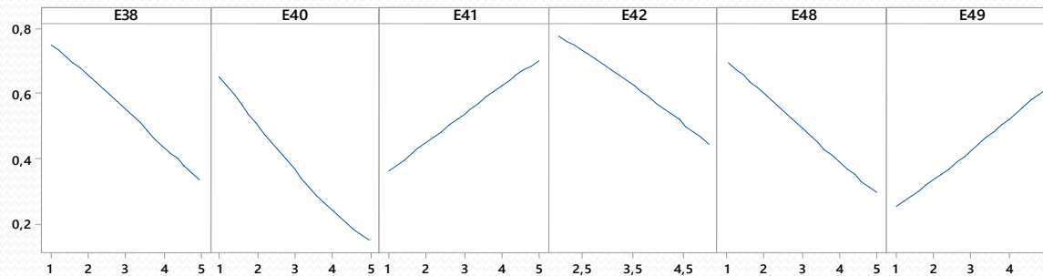
Main Effects Plot for E46_1 Fitted Probabilities
